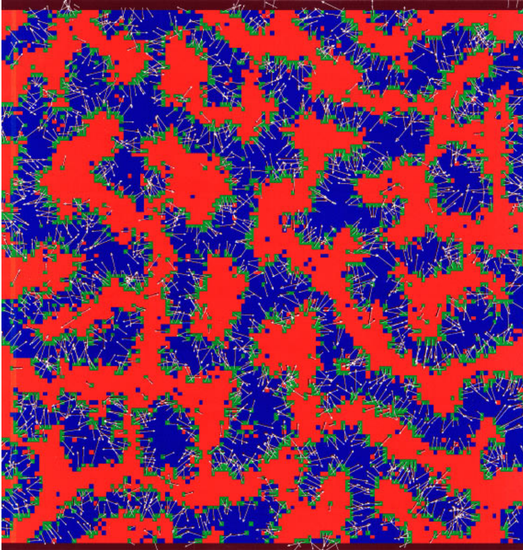
FIG. 7. (Color.) Bicontinuous microemulsion structure shown at time step 200 of a simulation with equal amounts of oil and water in the system. The arrows depict the direction of the amphiphile vectors: note that they always point from the oil to water domains, as we expect. Color code: blue, water; red, oil; green, surfactant.
